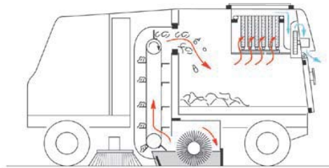
Dulevo Patented Mechanical-suction-filter system
