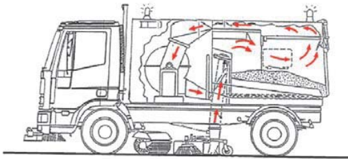
Traditional suction system
